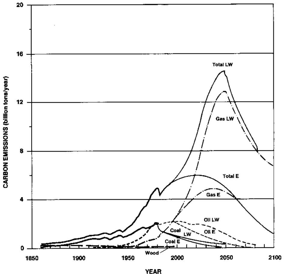
Fig. 8. Historic carbon emissions and projections for two methane-intensive scenarios.
